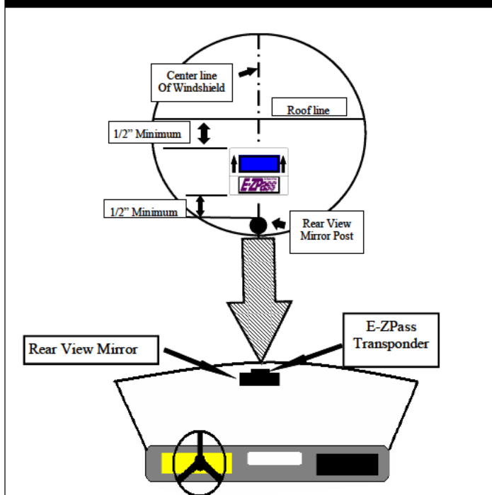
Fig. 2 Preferred E-ZPass Mounting Location
